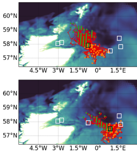
Locations of particles after 1 month that pass through the black box. Start (green)/ End (orange).
